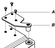
A. \frac{5}{16} " Hex-Head Hinge Screws B. Top Hinge
